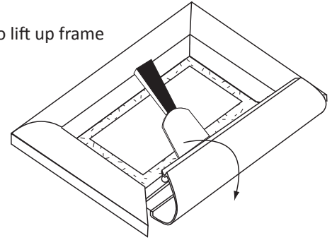
“Half Inch Bottom” piece for thicker graphics .251”-.500” Insert Thickness
